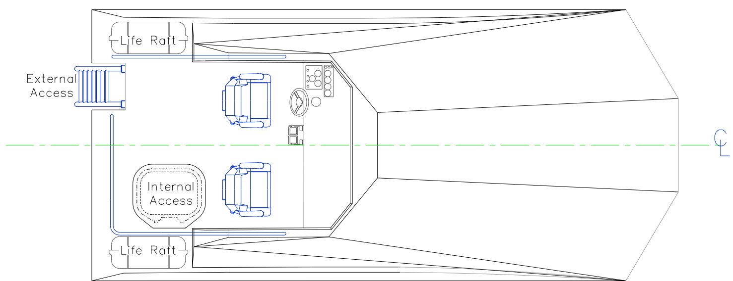
FLY BRIDGE PLAN
