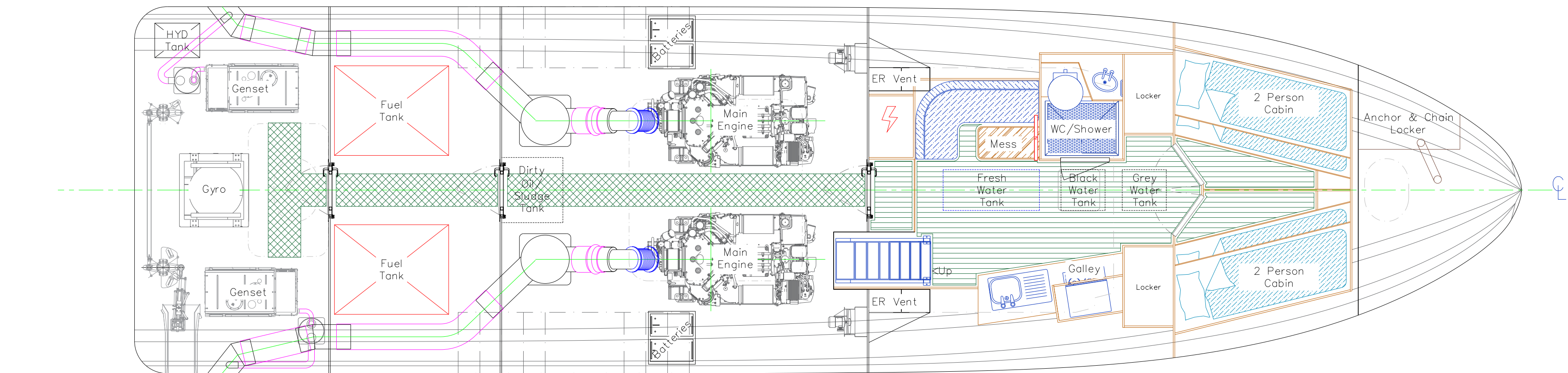
LOWER DECK PLAN
